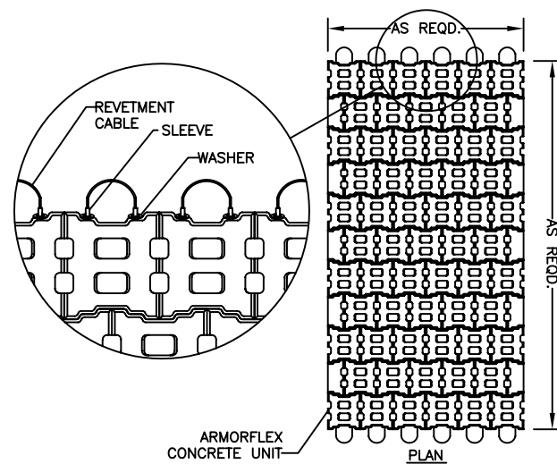
DETAIL II ARMORFLEX CL45 INTERLOCKING CONCRETE MATTRESS NOT TO SCALE
