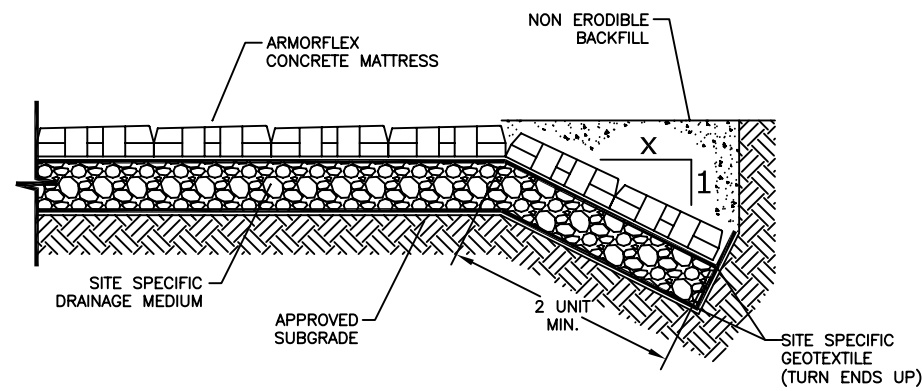
DETAIL IV ARMORFLEX CL45 TOP OF SLOPE NOT TO SCALE
