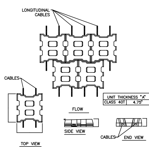
DETAIL I ARMORFLEX CL45 UNIT DIMENSIONS NOT TO SCALE
