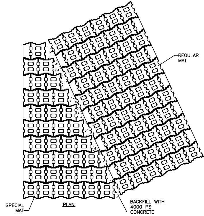
DETAIL IV ARMORFLEX CL45 ANGLE MATTRESS NOT TO SCALE
