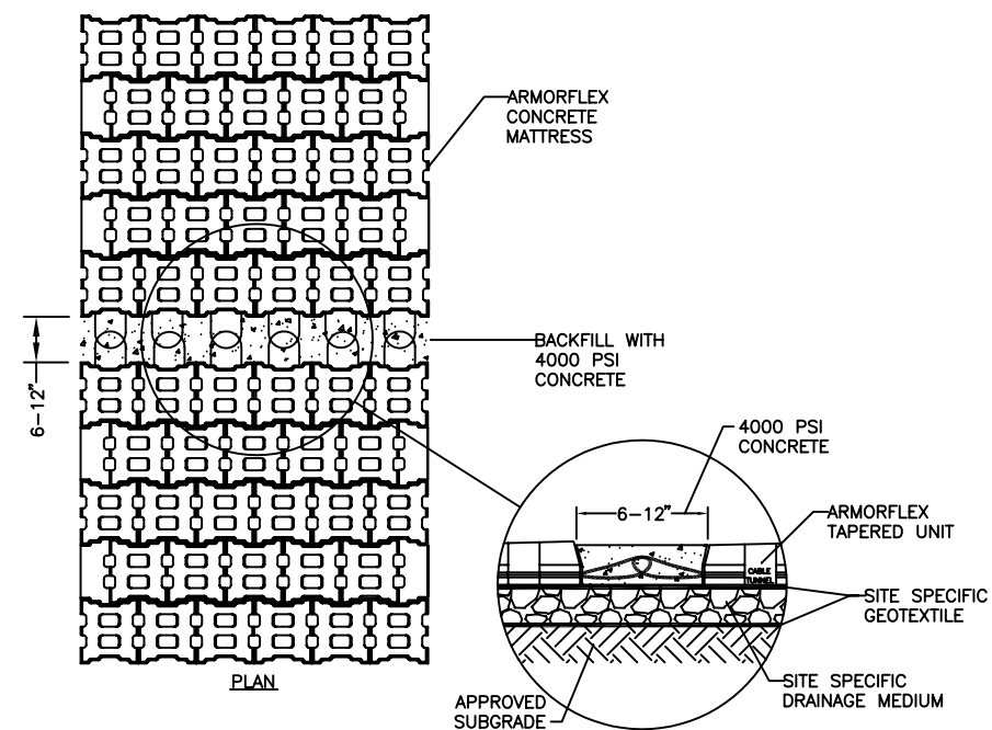
DETAIL III ARMORFLEX CL45 GROUT SEAM BETWEEN MATS NOT TO SCALE
