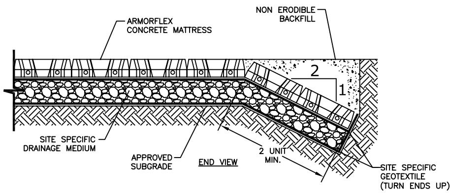
DETAIL V ARMORFLEX CL45 SIDE FLANK NOT TO SCALE
